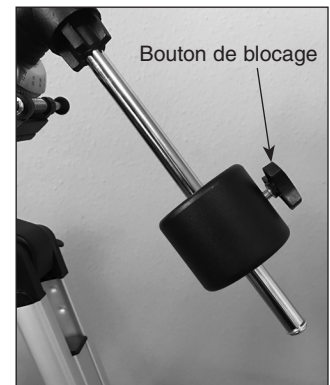
Figure 10. Le contreponds, installé.
